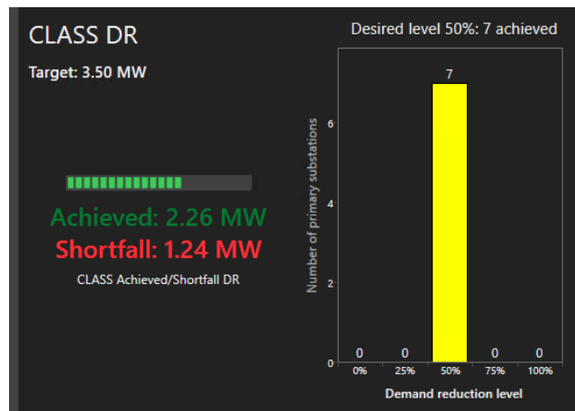
Figure 4-25 – QUEST Dashboard – CLASS target not satisfied
