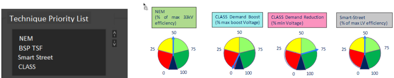
Figure 6-4 - TPL and BLENDS adjustment – NEM has priority over BSP TSF
