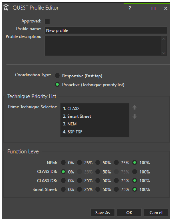
Figure 4-7 – QUEST PROFILE – Proactive coordination type
