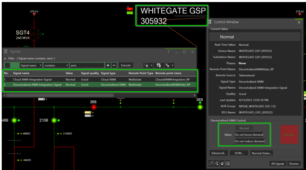
Figure 5-4 – QUEST integration with external ANM systems
