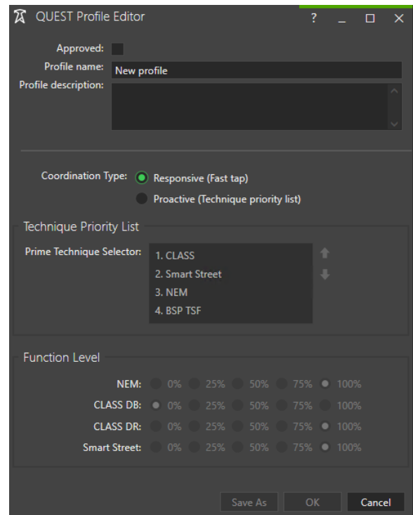
Figure 4-8 – QUEST PROFILE – Responsive coordination type
