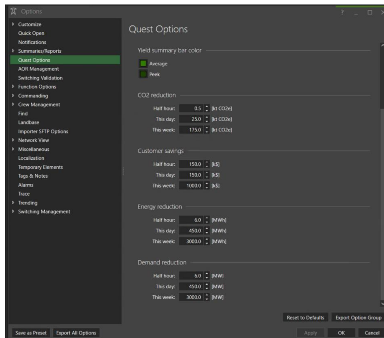
Figure 4-23 – QUEST Options related to QUEST Dashboard
