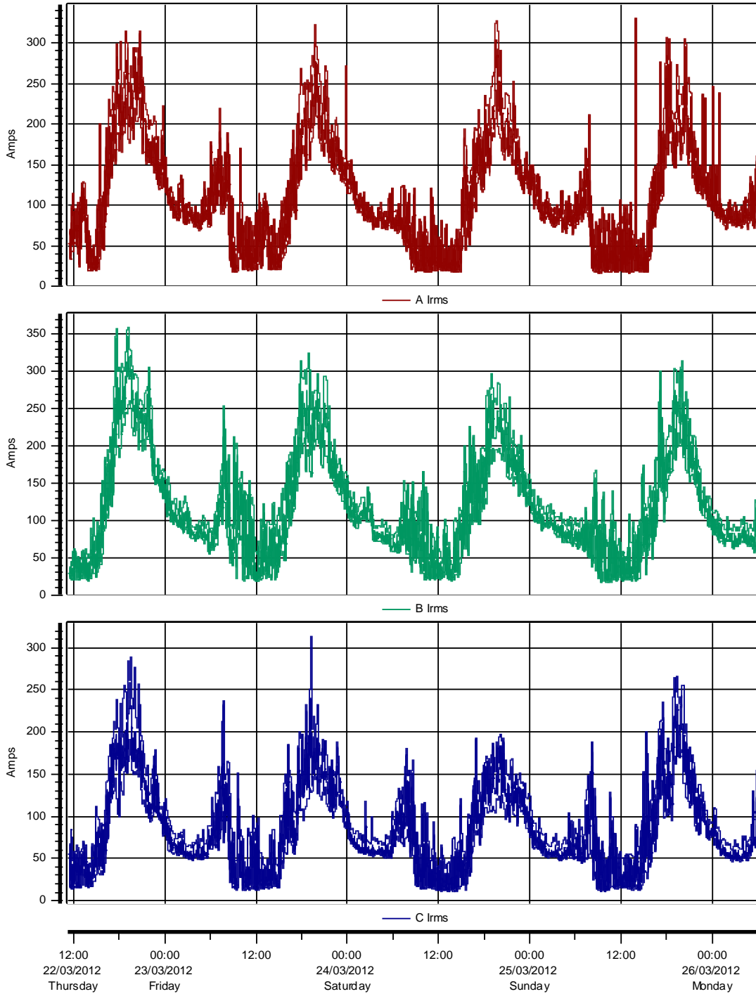
Timeplot Current RMS value
