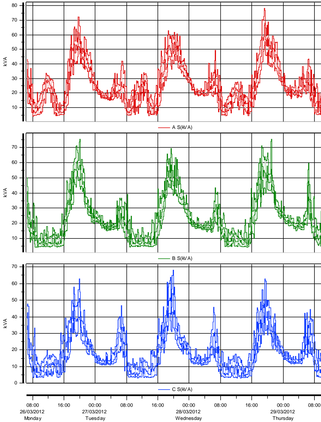
Timeplot Apparent power, S (VA)
