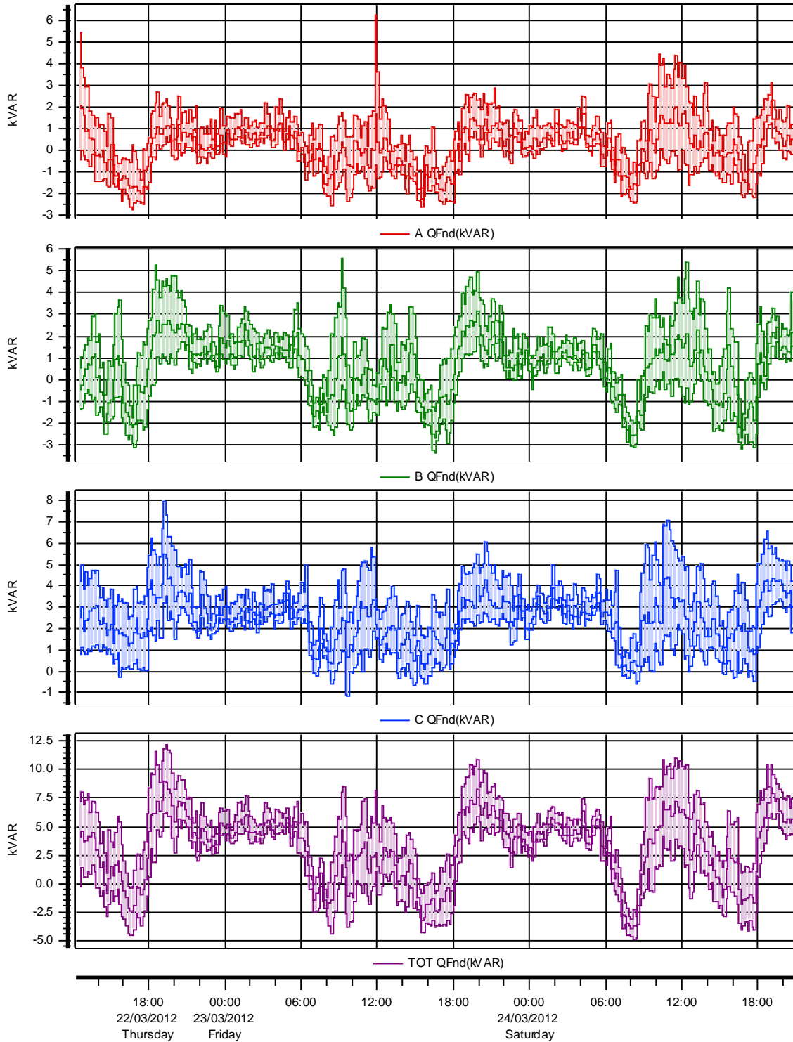
Timeplot Reactive power Q, at fund. freq. (VAR)
