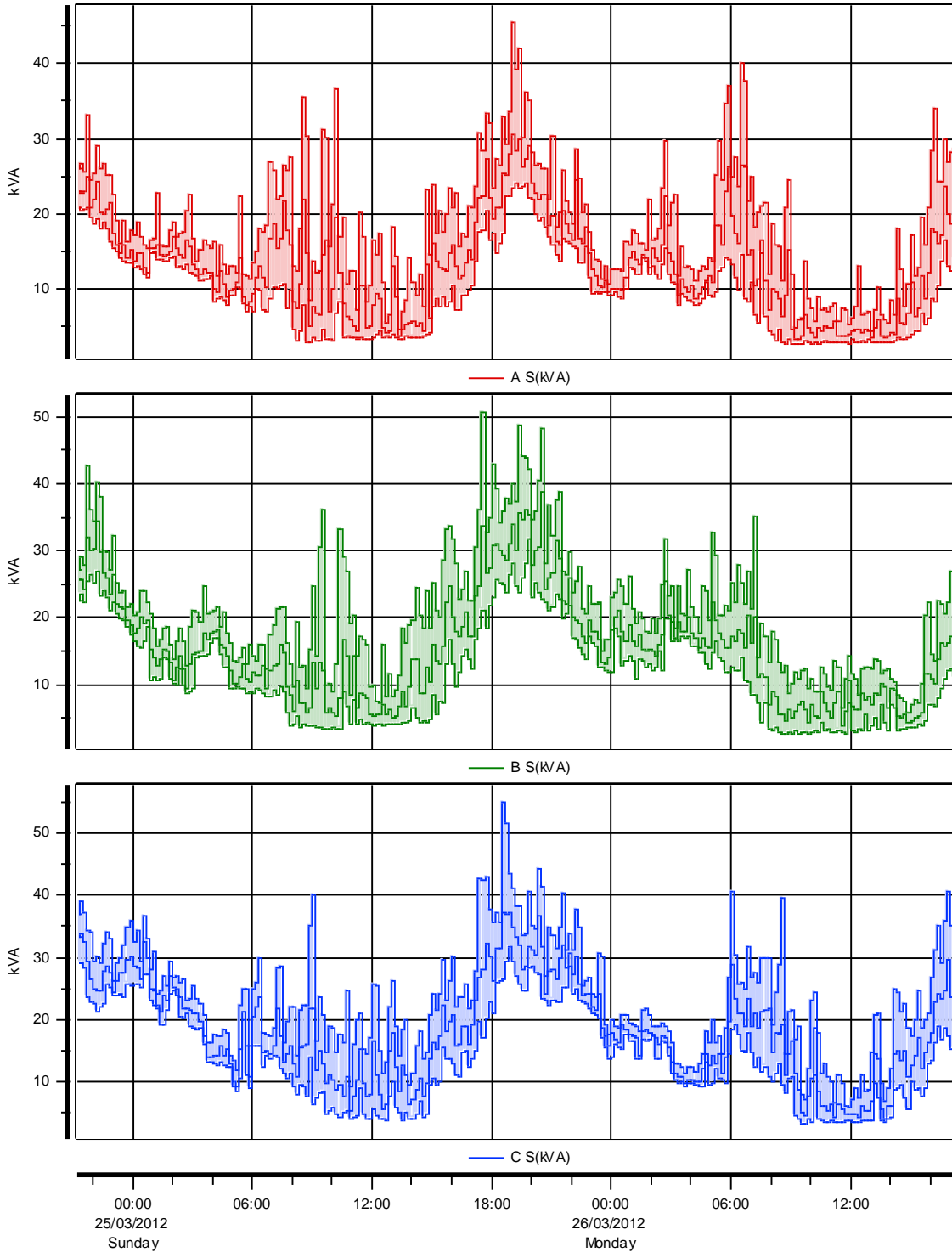
Timeplot Apparent power, S (VA)
