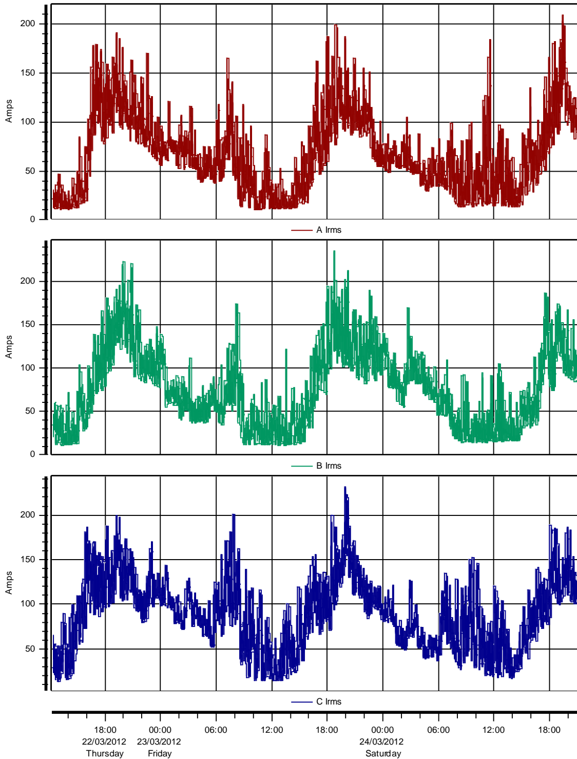
Timeplot Current RMS value
