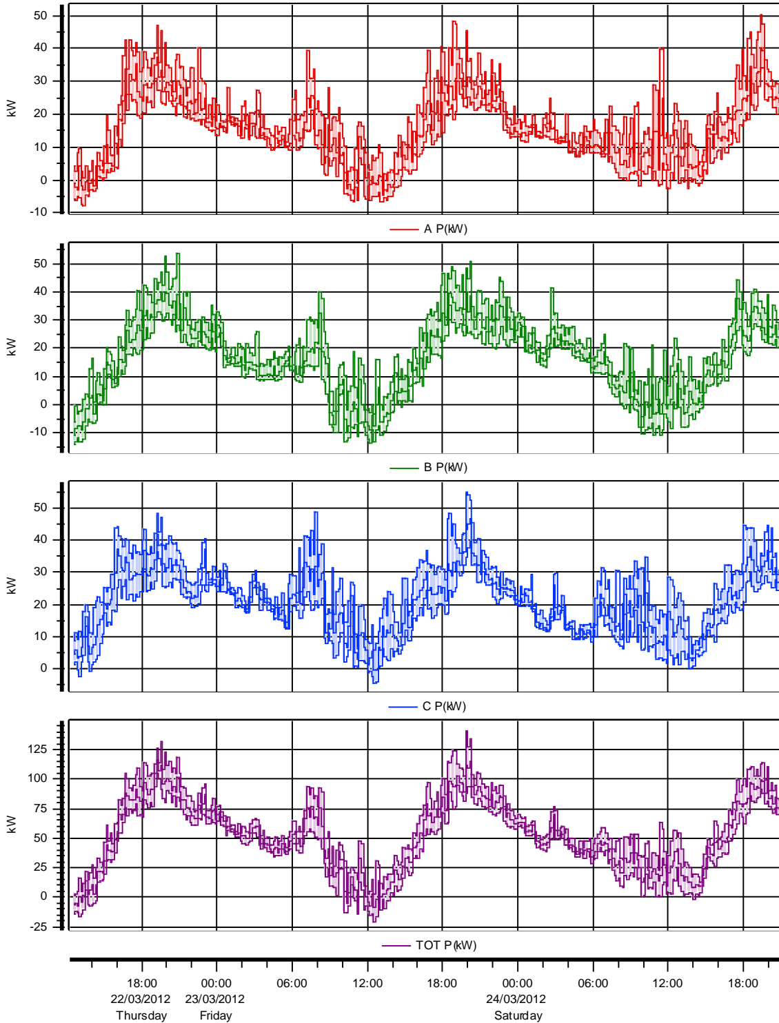
Timeplot Active power, P (W)
