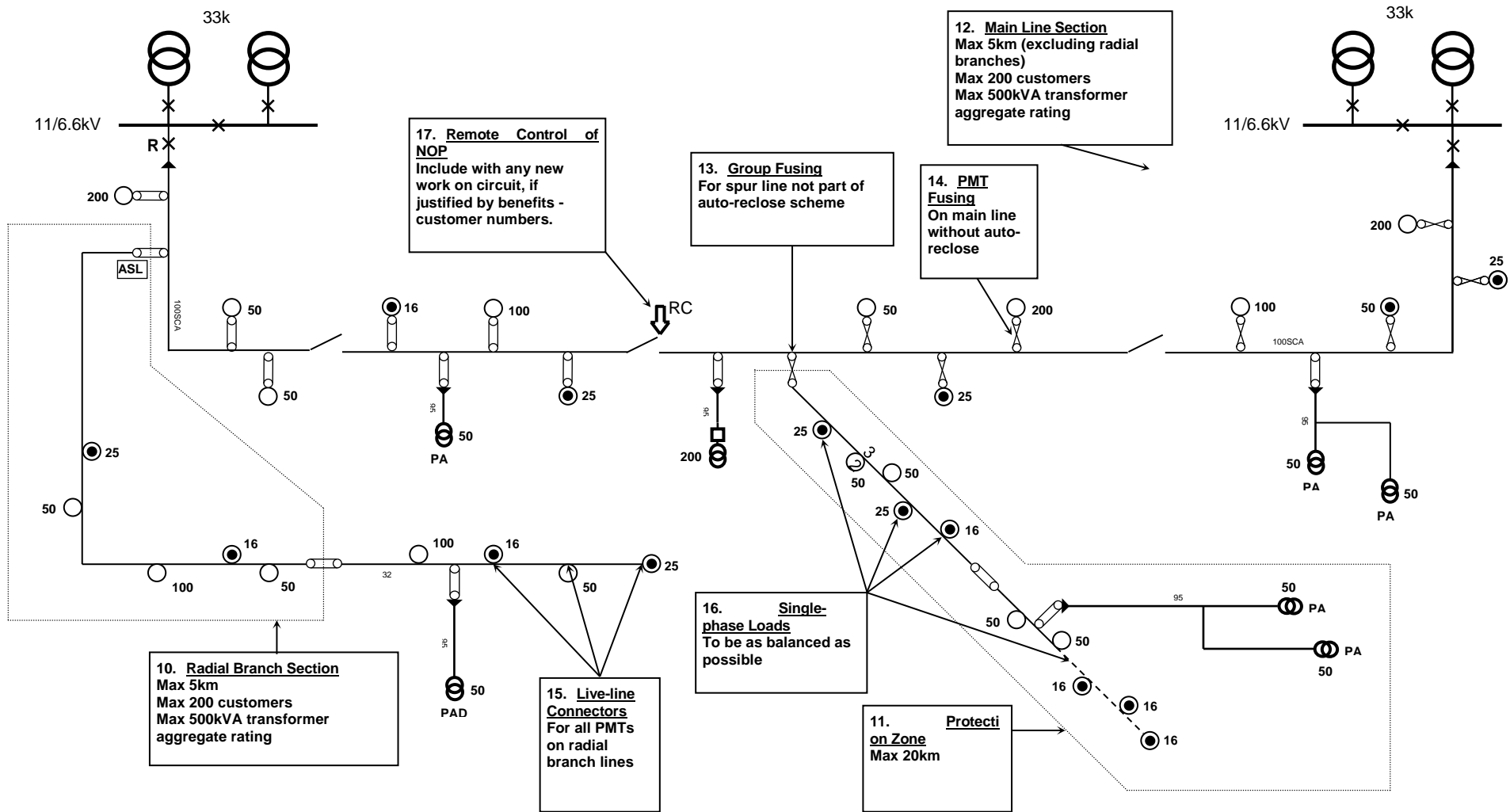
Figure A2 - Typical 11/6.6kV Overhead Network Arrangement
