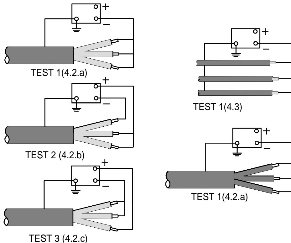
Diagram 1 - Test arrangements and sequences for belted cables (left), single core (right upper) and screened cables (right lower)
