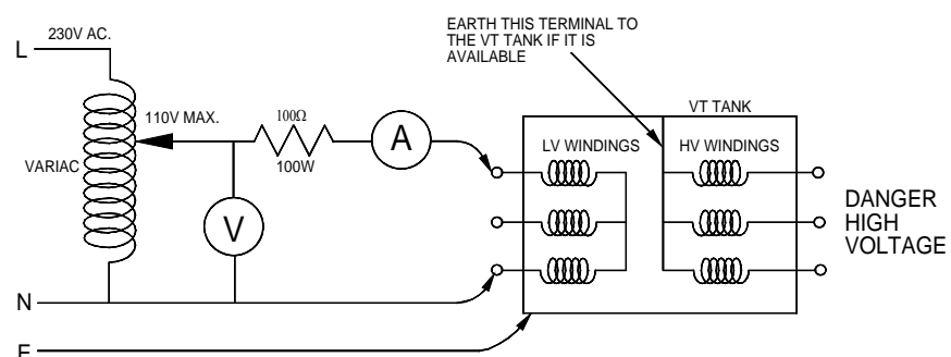
Diagram 4 - Test connections for voltage transformer if the low voltage winding star point is not available
