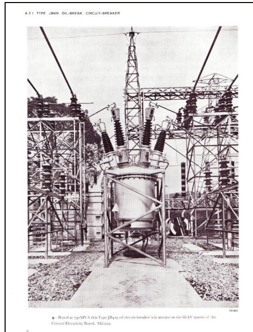
Photograph 2 - EHV 1950s UK manufactured oil circuit breaker (similar to that still operated in the UK) in service in Malaysia where ambient temperature can exceed 30°C
