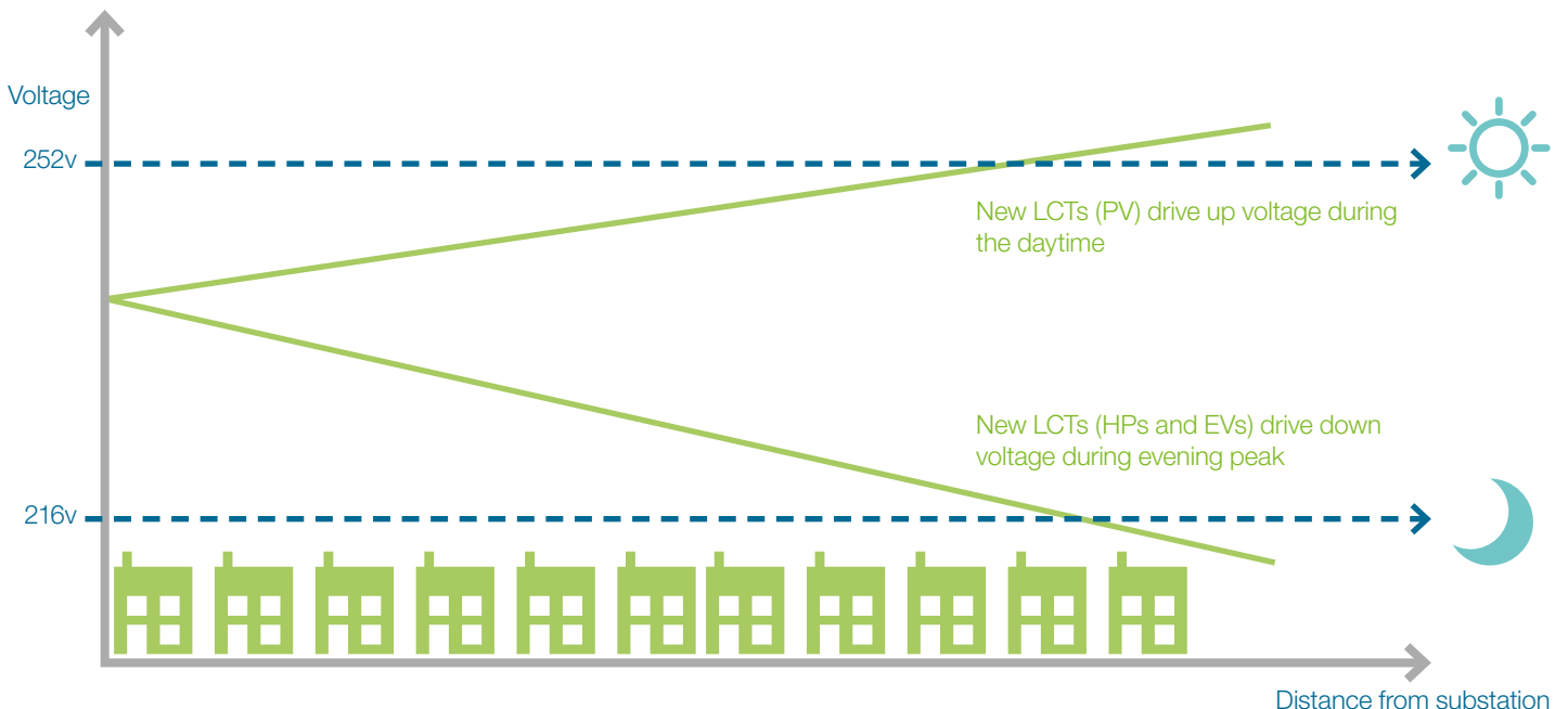
Impact of low carbon technologies on customer supply voltage
